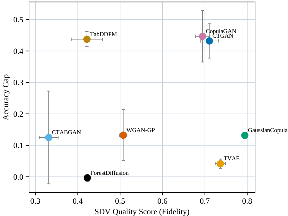
Alzheimer's: SDV Quality Score (Fidelity) vs Accuracy Gap
